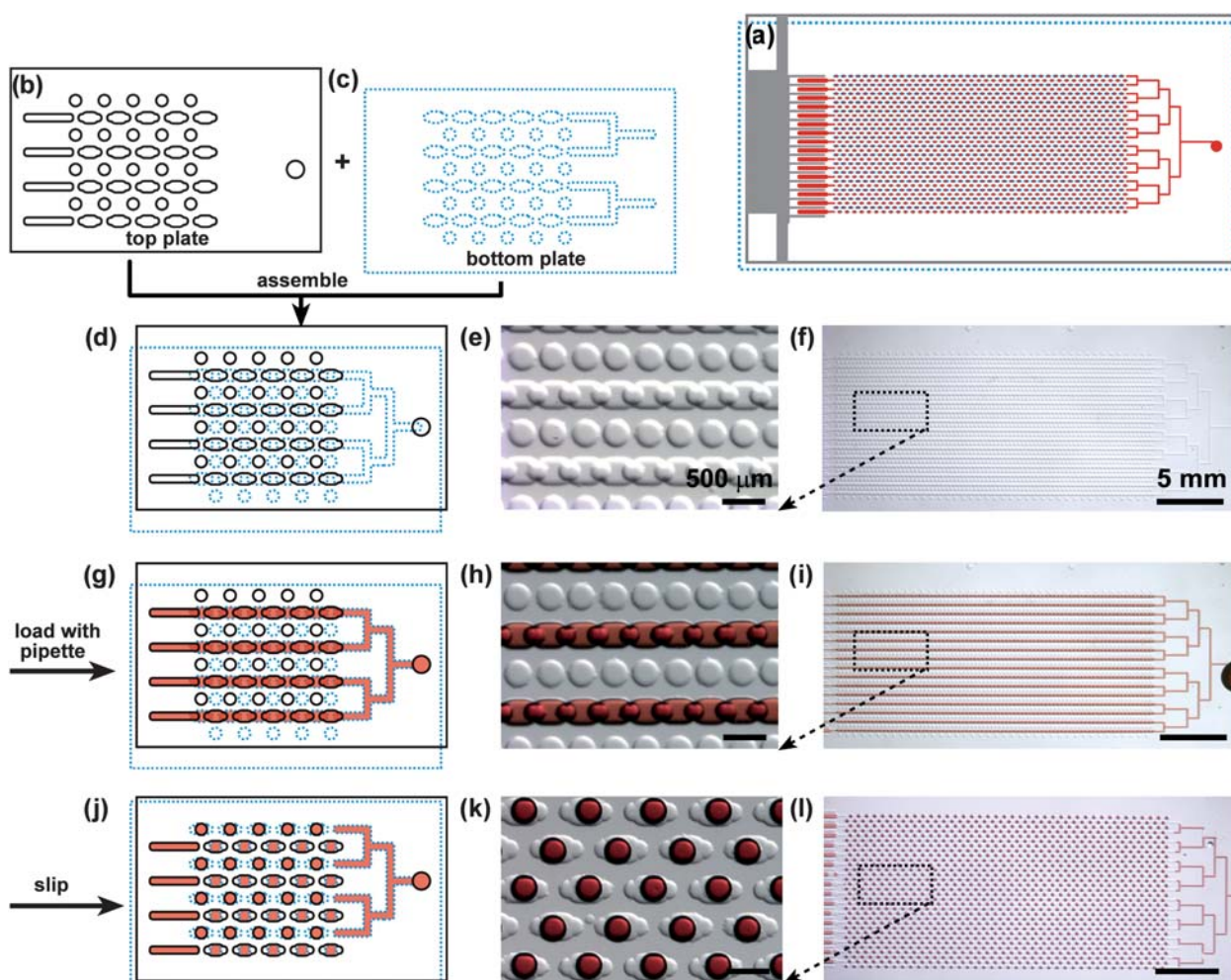
Fig. 1 Schematic drawing and bright field images show the design and mechanism of the SlipChip for digital PCR. The top plate is outlined with a black solid line, the bottom plate is outlined with a blue dotted line, and red represents the sample. (a) Schematic drawing shows the design of the entire assembled SlipChip for digital PCR after slipping. (b) Schematic drawing of part of the top plate. (c) Schematic drawing of part of the bottom plate. (d–f) The SlipChip was assembled such that the elongated wells in the top and bottom plates overlapped to form a continuous fluidic path. (g–i) The aqueous reagent (red) was injected into SlipChip and filled the chip through the connected elongated wells. (j–l) The bottom plate was slipped relative to the top plate such that the fluidic path was broken up and the circular wells were overlaid with the elongated wells, and aqueous droplets were formed in each compartment. (d, g and j) Schematic of the SlipChip; (e, h and k) zoomed in microphotograph of the SlipChip; (f, i and l) microphotograph of the entire SlipChip.
